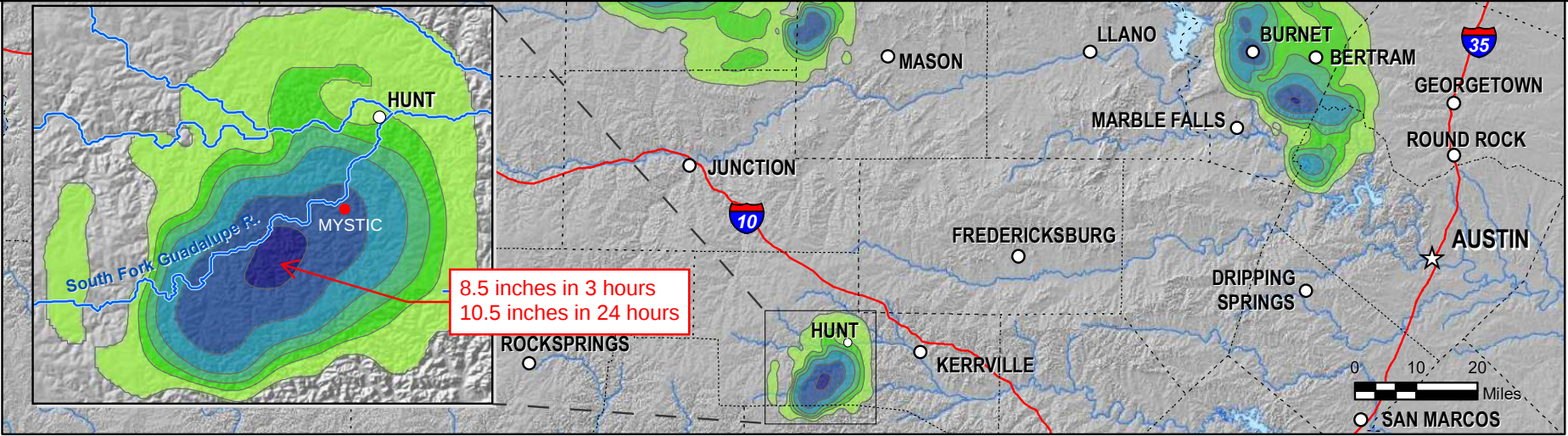
Hill Country, Texas, 3-6 July 2025 Annual Exceedance Probabilities (AEPs) for the Highest 3-hour Rainfall Period
